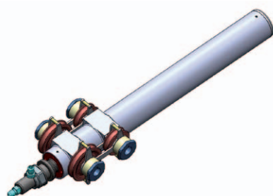
Titanium twin cylinder: n.2 double acting cylinder move together in a common tube. Bore (each): 25mm Stroke: 190mm Working pressure: 700 bar Extreme light weight and compact design.
